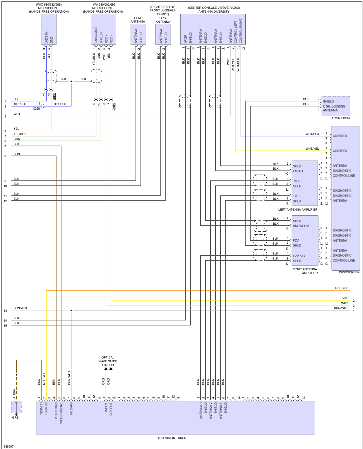
Fig 2: Navigation Circuit, W/ Burmester (2 of 4)
