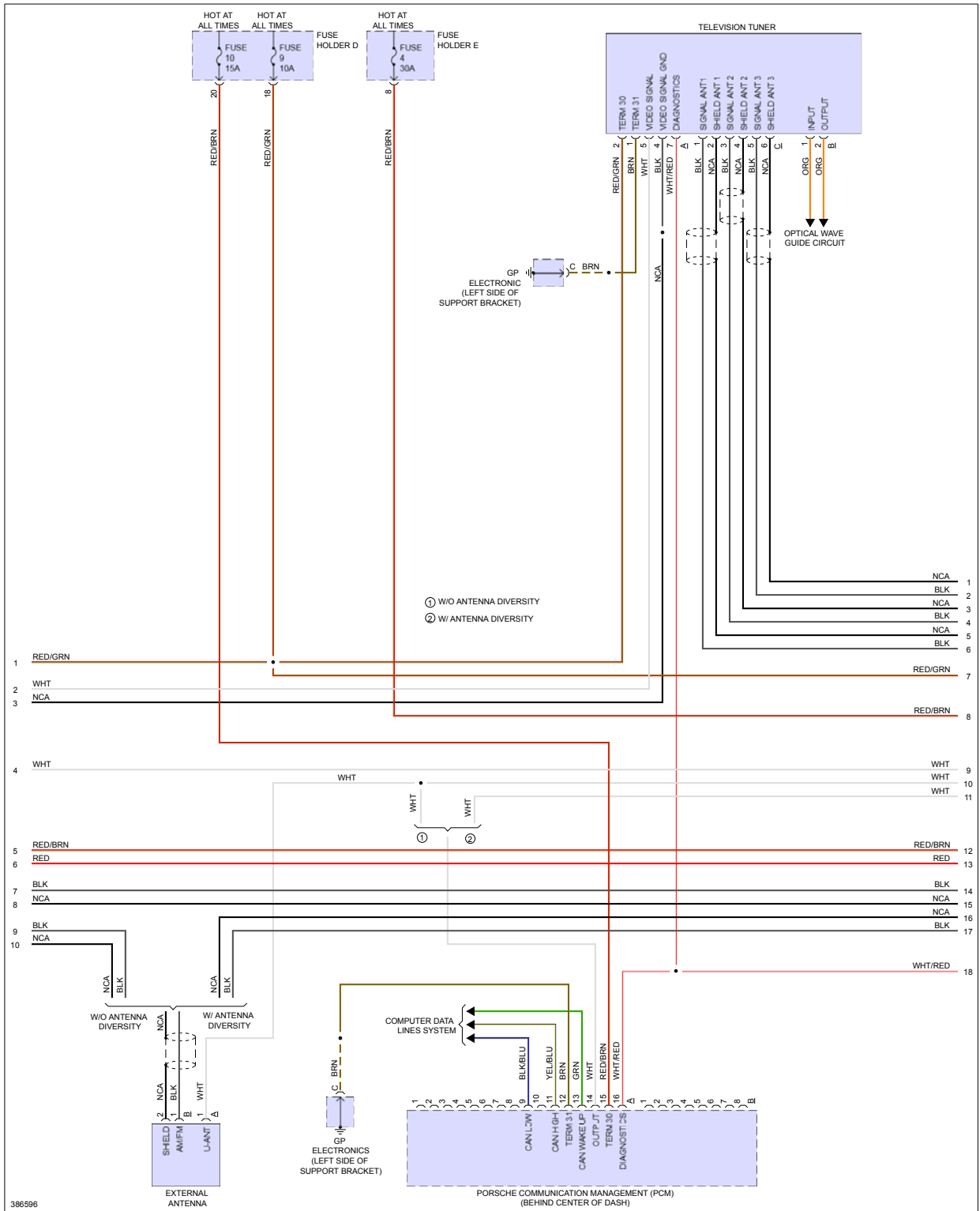
Fig 7: Navigation Circuit, W/ Turbo W/ Bose (2 of 4)
