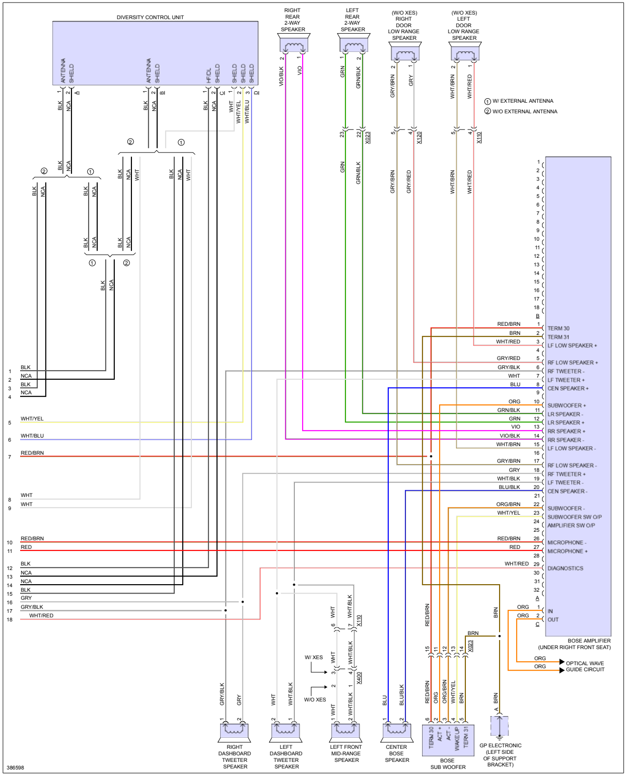
Fig 9: Navigation Circuit, W/ Turbo W/ Bose (4 of 4)
