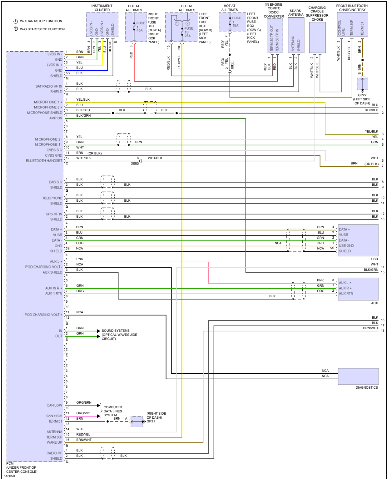
Fig 3: Premium Radio Circuit, W/ ASK (1 of 4)
