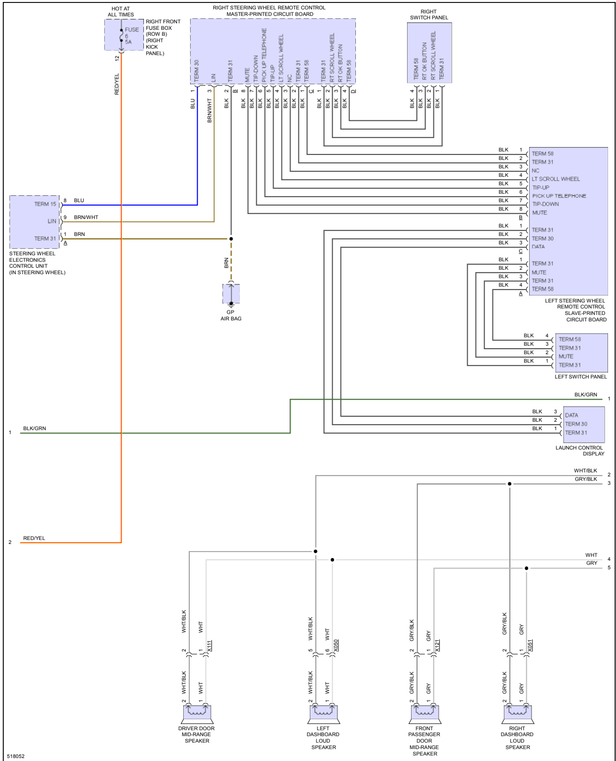
Fig 5: Premium Radio Circuit, W/ ASK (3 of 4)
