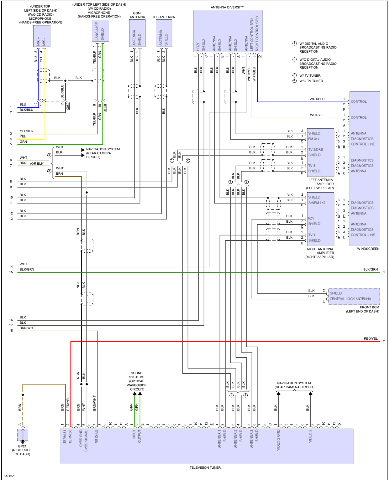
Fig 4: Premium Radio Circuit, W/ ASK (2 of 4)
