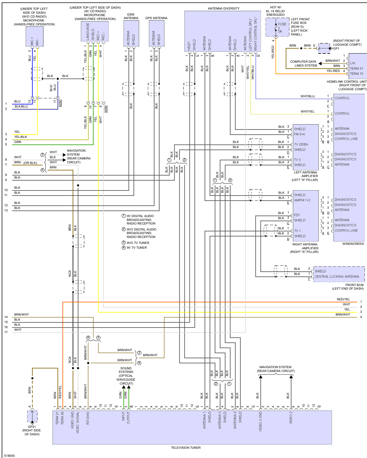
Fig 8: Premium Radio Circuit, W/ Bose (2 of 4)
