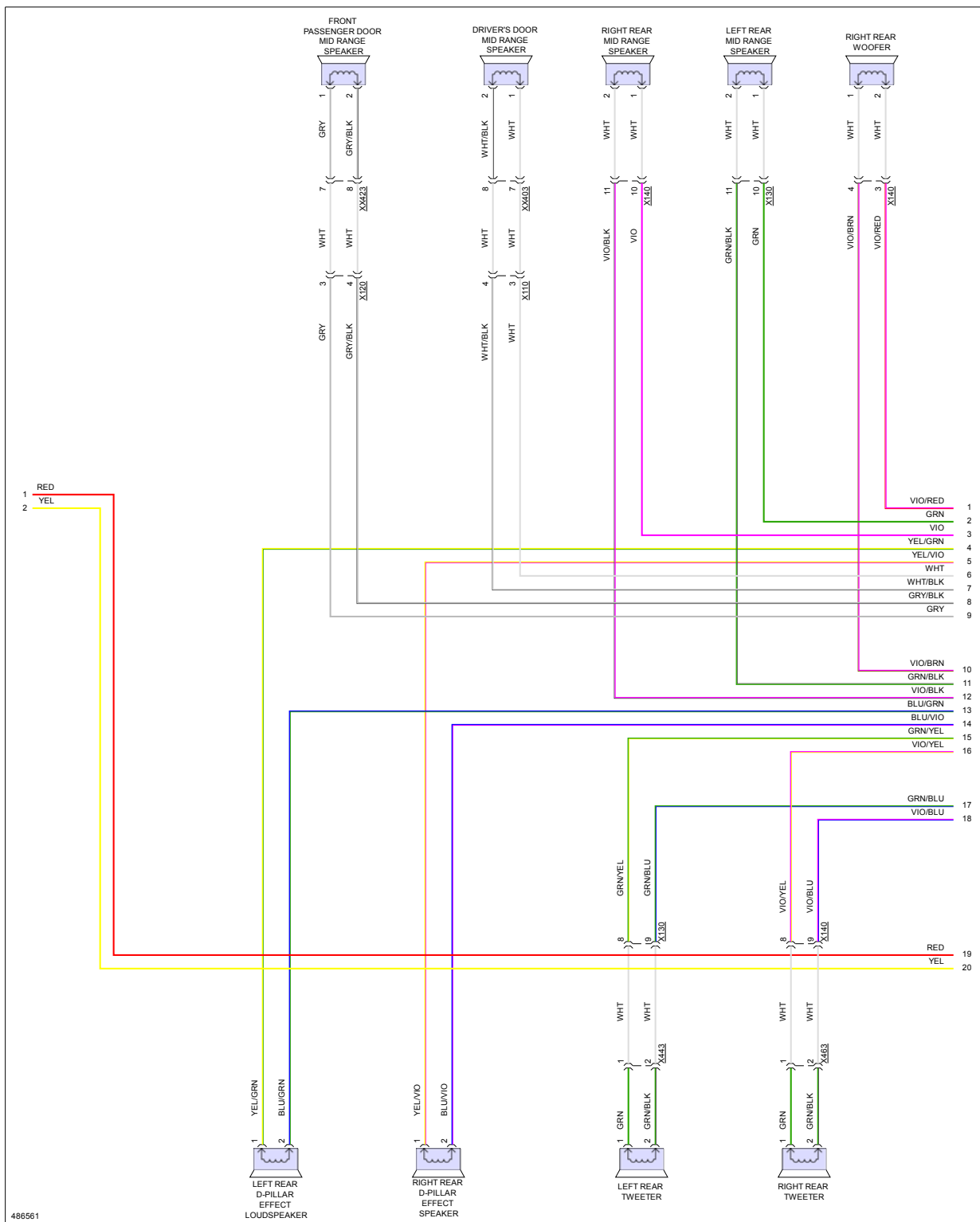
Fig 11: Navigation Circuit, W/ Burmester (3 of 4)
