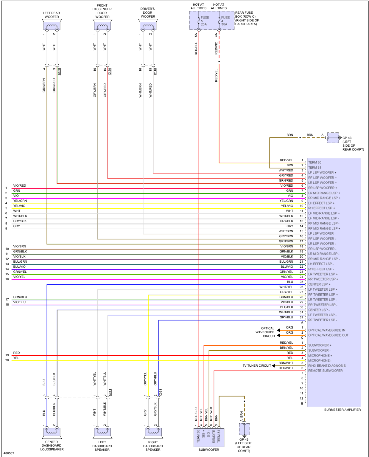
Fig 12: Navigation Circuit, W/ Burmester (4 of 4)
